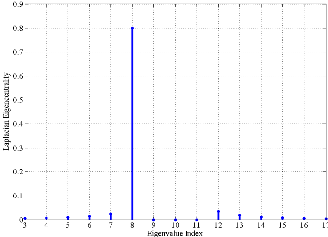
Fig. 5. Eigenspectrum of node six at time zero of the simulation
