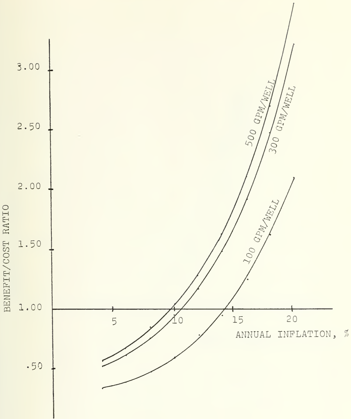
FIG. 9 BENEFIT/COST RATIO vs. ANNUAL FUEL INFLATION RATE RUN I (UPPER BOUND) 150°F WELL OUTPUT.
