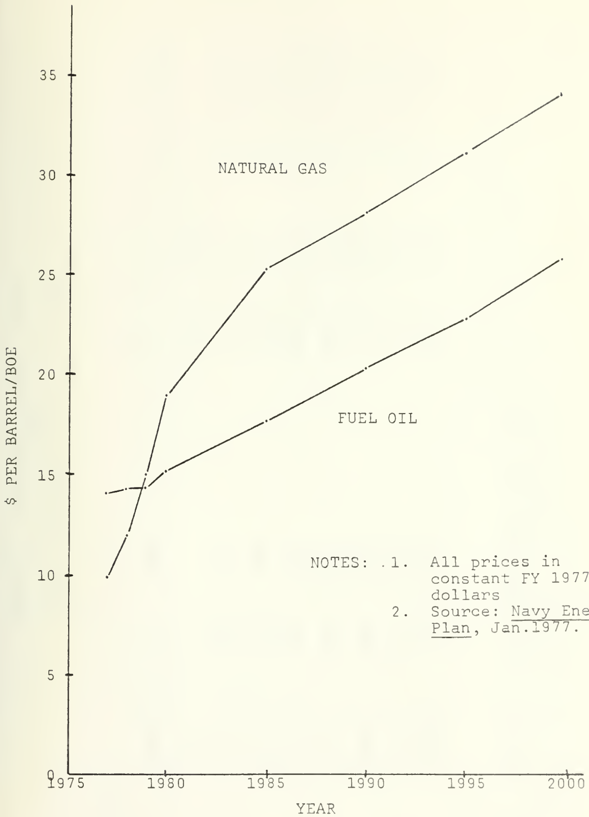
Fig. 8 PROJECTED FUEL PRICES FY 1977 TO FY 2000
