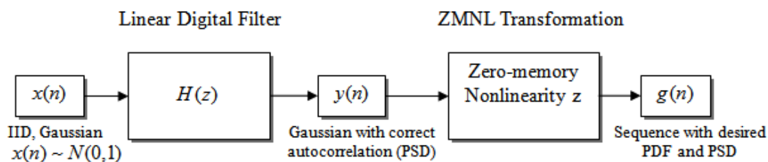
Figure 4. General process for generating signals with a user defined PDF and PSD. From [8].
