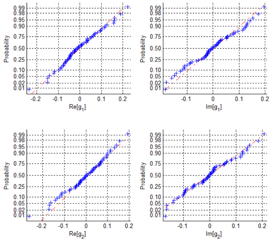
Figure 16. Normal distribution plots of the first two targets in the target realization set. Left column: normal distribution plots of the real values of the first two targets; right column: normal distribution plots of the imaginary values of the first two targets.
