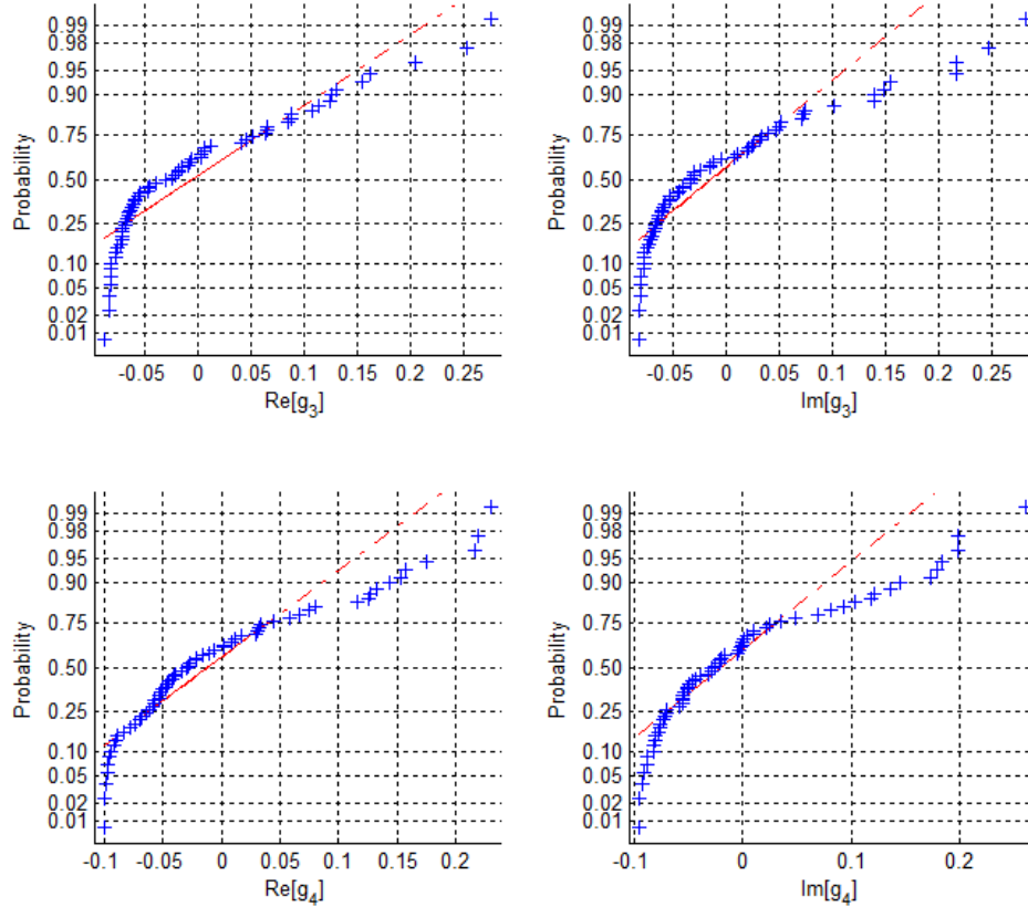
Figure 25. Normal distribution plot of one particular realization of the second target hypothesis set. The plots for the real values of the last two targets are presented on the left column and the plots for the imaginary values of the last two targets are presented on the right column.
