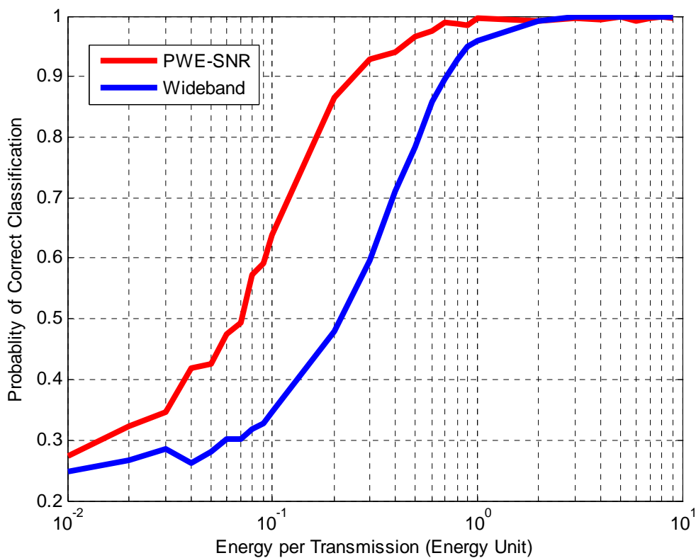
Figure 35. Classification performance curves of the optimized SNR illumination waveform and a traditional wideband waveform with the implementation of the NGCCR system for ten transmissions. Target distributions: Rayleigh, exponential, Gamma, log-normal. Monte Carlo setup: 50 target realizations; ten noise realizations. NGCCR setup: 40 online target realizations for the ensemble averaging.
