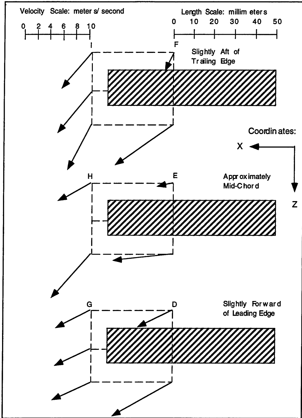
Figure IV.5 Profile View (X-Z Plane) of Flow Velocity Vectors at Selected Test Points
