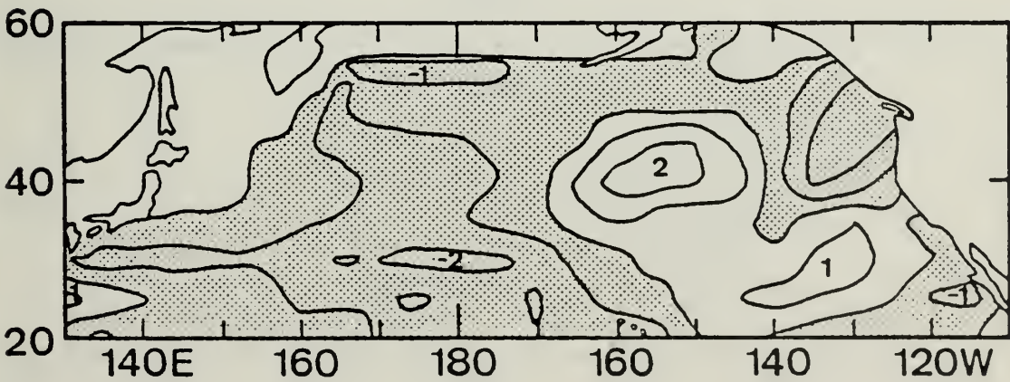
Figure 25. Subsample record correlations (nondimensionalized by \sigma_k^* ) between SST and (U_*^3)_{HL} for +1 month lag and starting months January (top), February (middle), and March (bottom). Contour interval is 1 and shading indicates negative correlations.
