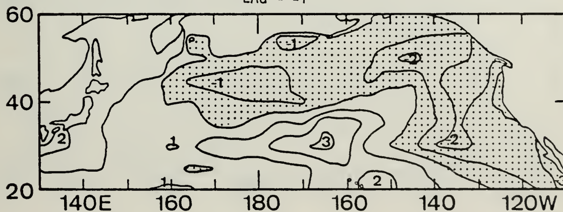
Figure 18. Same as Fig. 3 except for (CURL Z τ)TOT.
