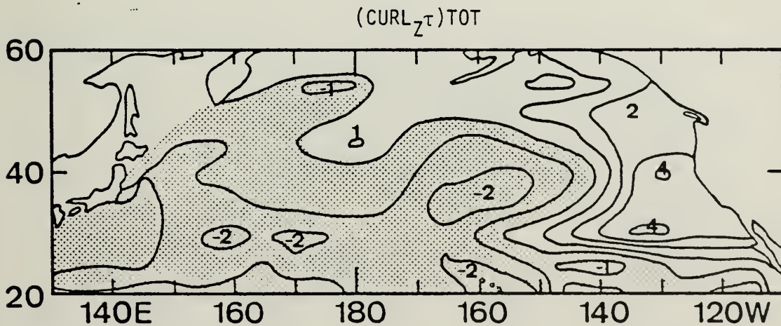
Figure 21. Normalized correlations at zero lag between \partial/\partial t SST and (\text{CURL}_{z\tau})_H , (\text{CURL}_{z\tau})_{HL} and (\text{CURL}_{z\tau})_{TOT} . Contour interval is 1 and shaded areas denote negative correlations.
