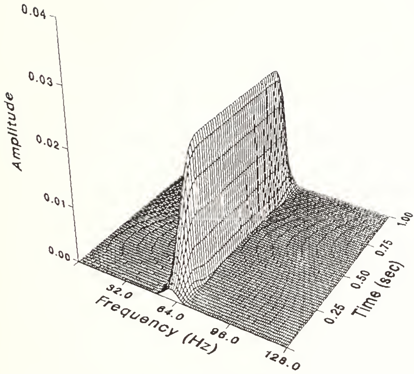
(a) s(t) = \cos(2\pi 60 t)
