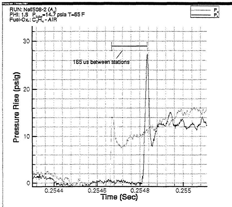
Figure A-10. Time Elapsed for Shock Wave Passage between 2 Pressure Sensors. Error in time measurement is \pm 1.6 \mu s .
