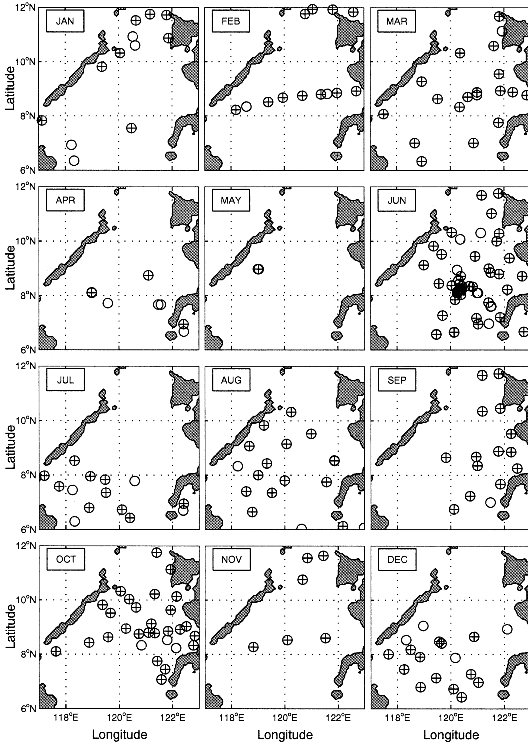
FIG. 3. Monthly CTD stations (denoted by "o") and the stations with BL occurrence ( H_D < H_T ; denoted by "+") in the Sulu Sea.
