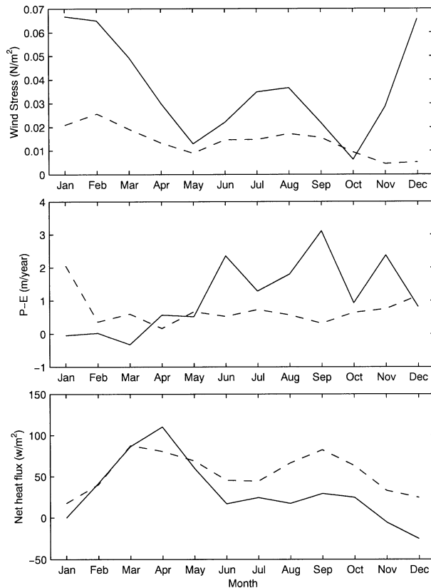
FIG. 9. Monthly mean COADS (a) surface wind stress ( N m^{-2} ), (b) P - E ( m yr^{-1} ), and (c) net heat flux ( W m^{-2} ) averaged over the Sulu Sea (solid curve) and the Celebes Sea (dashed curve).
