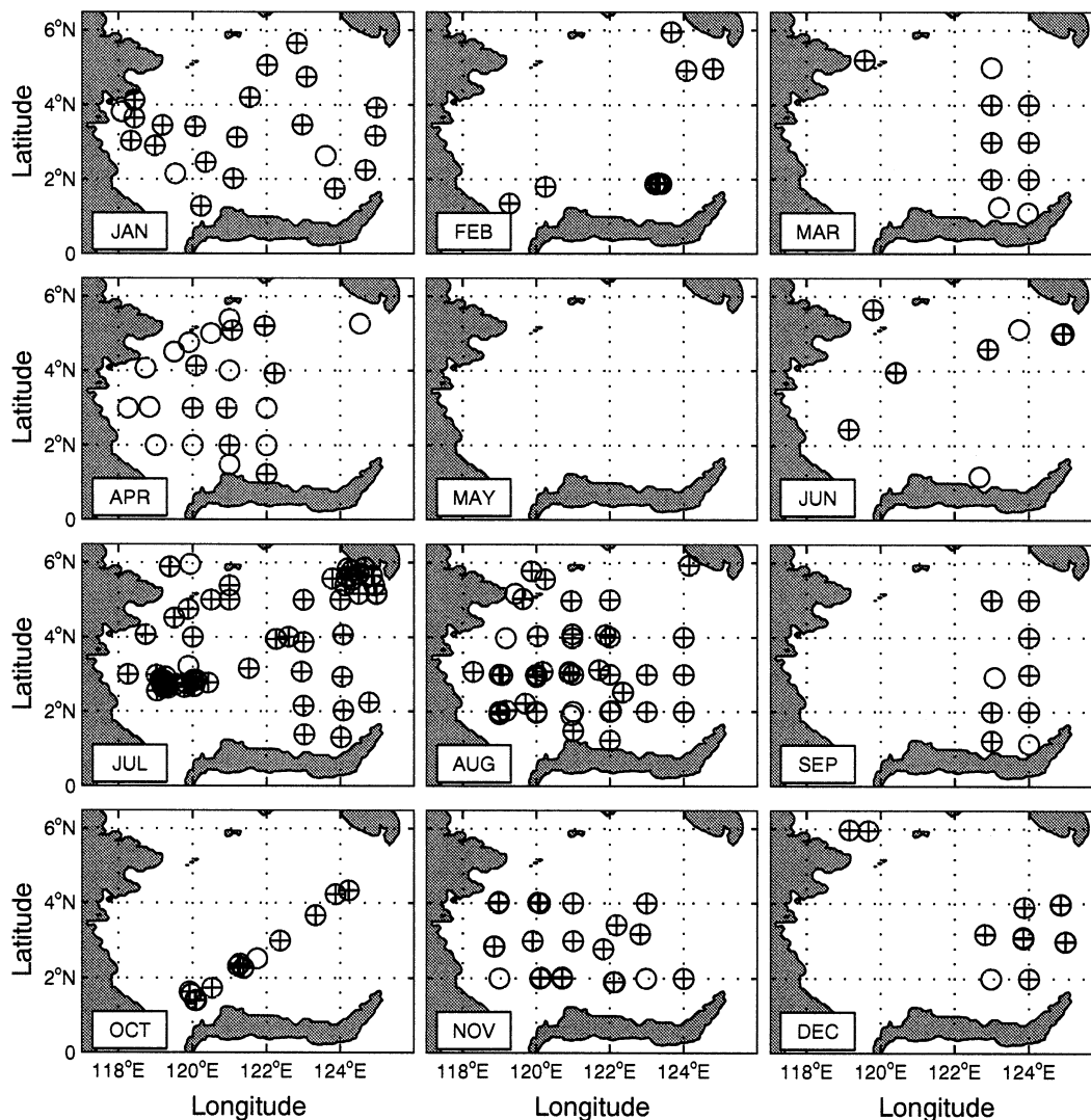
FIG. 6. Monthly CTD stations (denoted by “o”) and the stations with BL occurrence ( H_D < H_T ; denoted by “+”) in the Celebes Sea.
