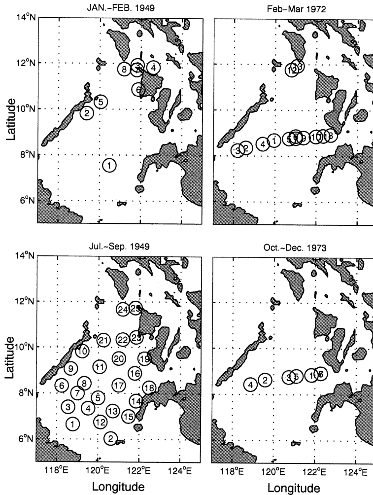
FIG. 4. CTD stations in the Sulu Sea for the four selected periods: (a) Jan–Feb 1949, (b) Feb–Mar 1972, (c) Jul–Sep 1949, and (d) Oct–Dec 1973.
