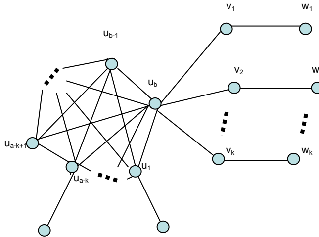
Figure 8. The Graph G in Theorem 2 [4]
