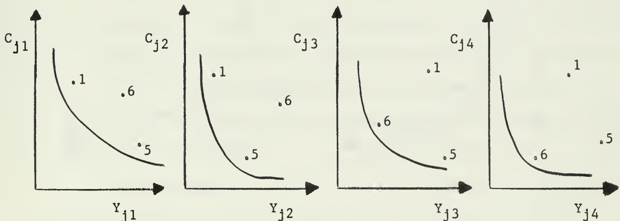
Figure 5.2 PLOT OF THREE DOMINATING ALTERNATIVES
