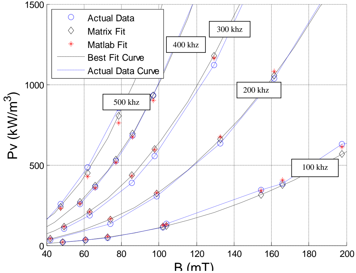
Figure 40: CPL graph using MATLAB Method
