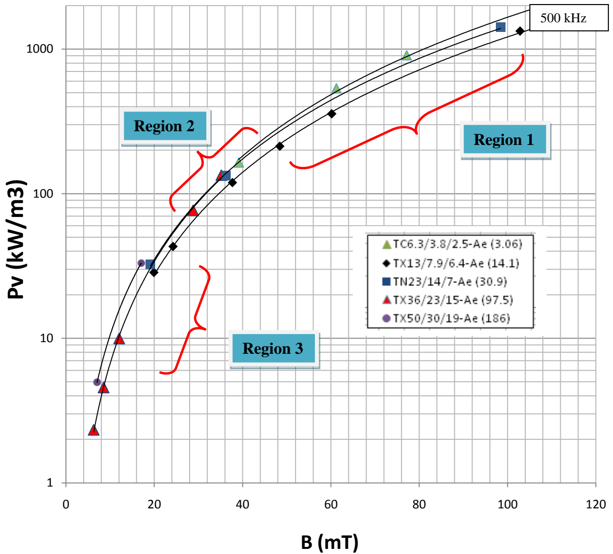
Figure 36: Core Area CPL Losses for 500 khz
