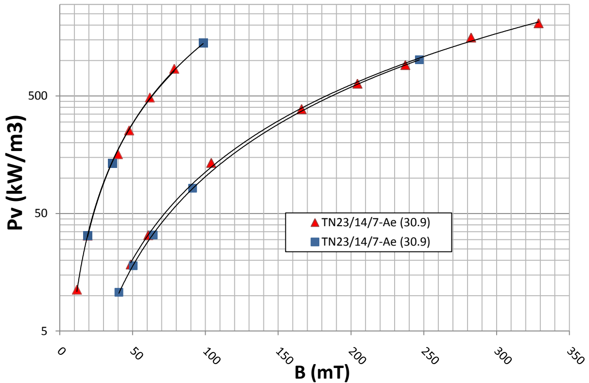
Figure 33: 3F3 TN 23/14/7 same size core lot Variability
