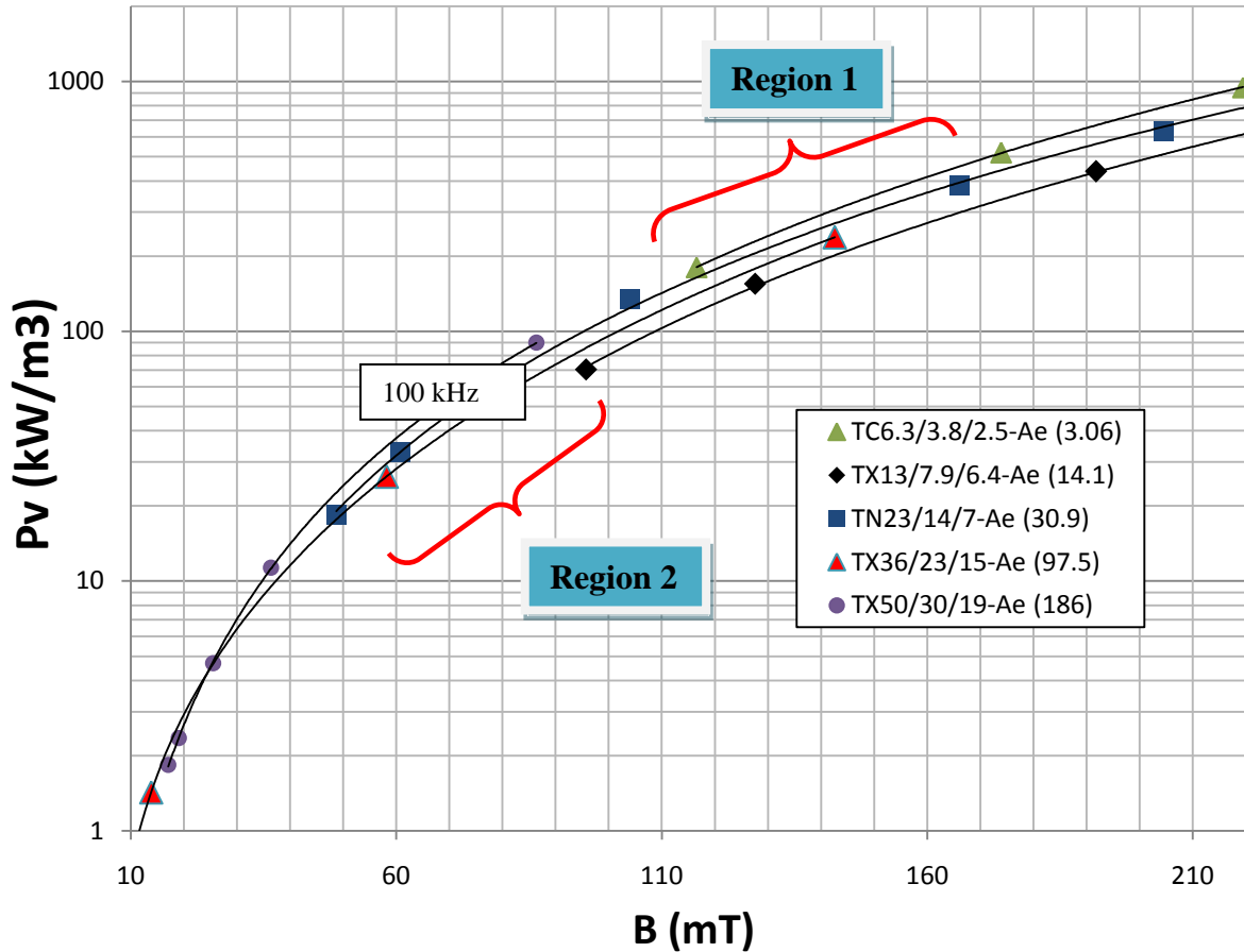
Figure 35: Core Area CPL Losses for 100 khz
