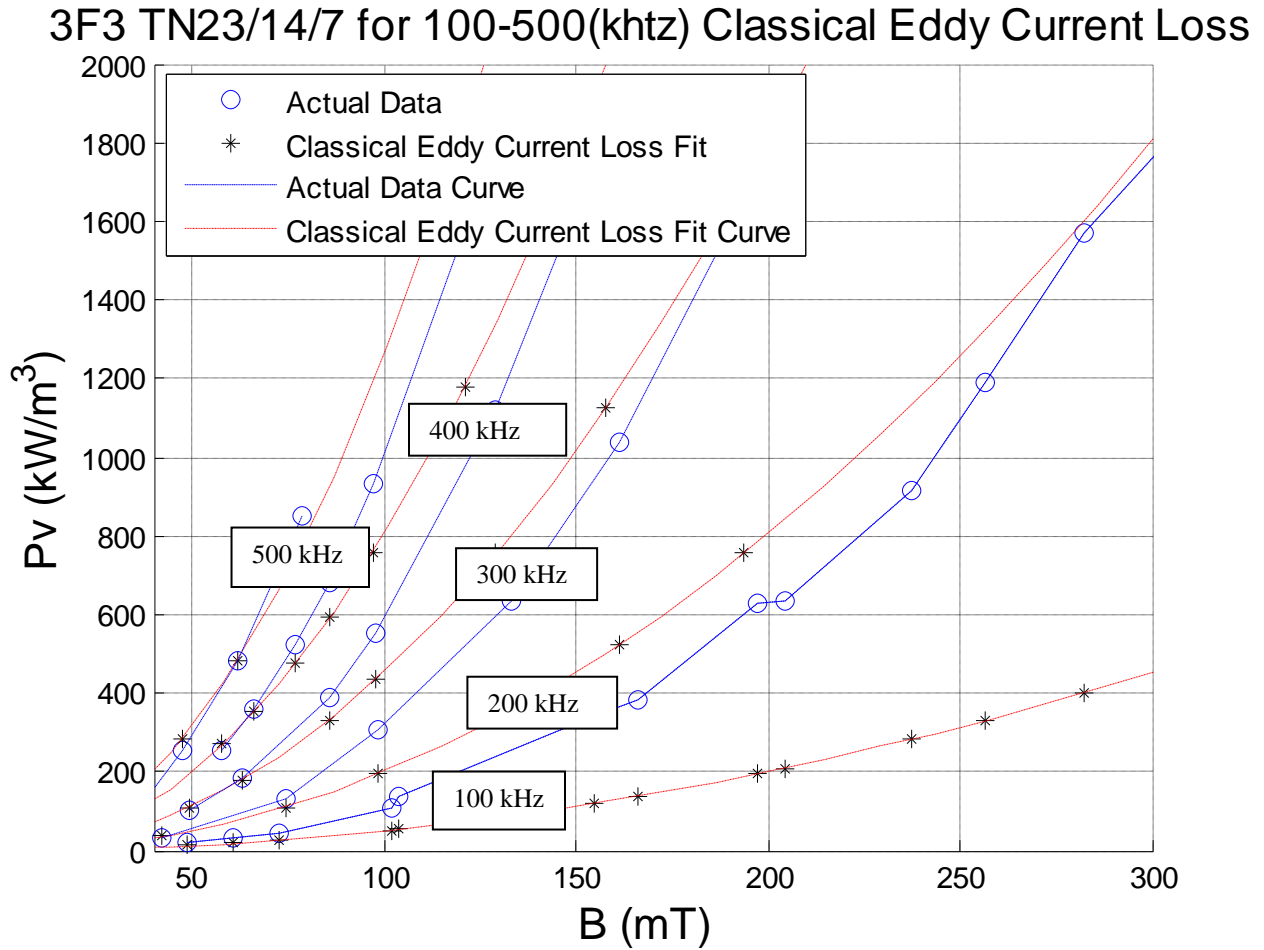
Figure 50: Classical Eddy Current Loss Equation for 100-500 kHz Data
