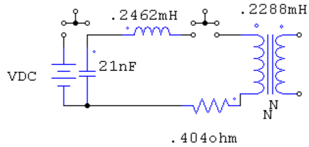
Figure 8: Preconditioning Circuit values
