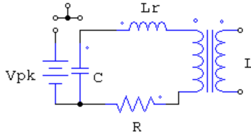
Figure 7: Preconditioning Circuit
