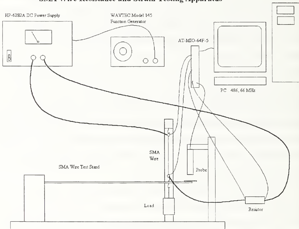
Figure 4.1 : SMA Resistance/Strain - Current Test Apparatus.
