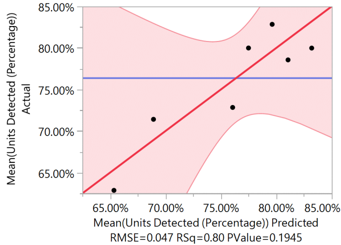
Figure 16. Actual vs. Predicted Plot: UUV Detection
